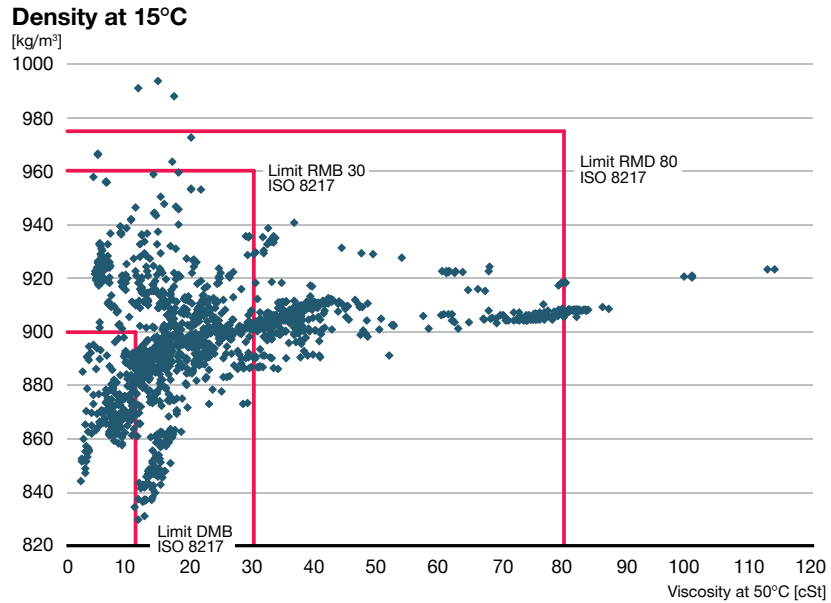
Fig. 9: Density, kg/m 3 at 15°C and viscosity, cSt at 50°C of 0.10% S ULSFO-RM supplied in 2015-2016. Data: LR FOBAS. Interpretation and evaluation: MAN ES
