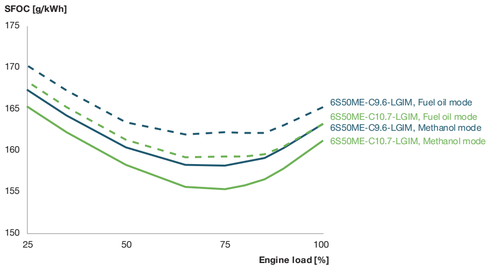
Fig. 3: SFOC for 6S50ME-C10.7-LGIM and 6S50ME-C9.6-LGIM engines in methanol and fuel oil modes (at 9,200 kW and 111 rpm)
