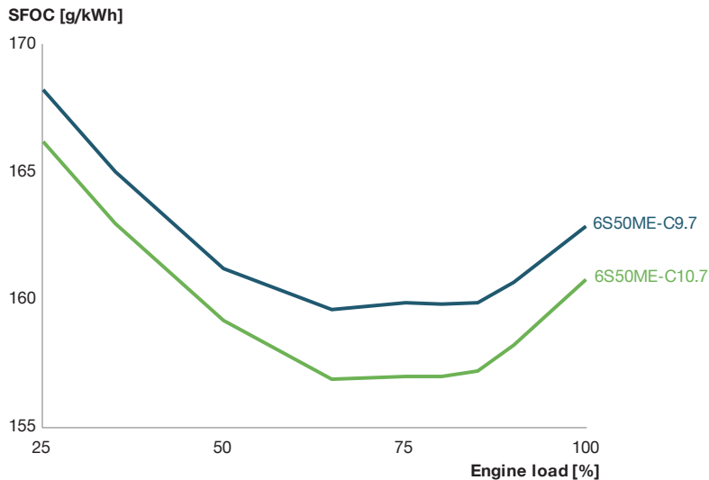
Fig. 2: SFOC for 6S50ME-C10.7 and 9.7 engines in Tier II high-load operation (at 7,000 kW and 86 rpm)
