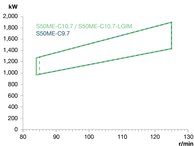
Fig. 1: Layout diagrams
